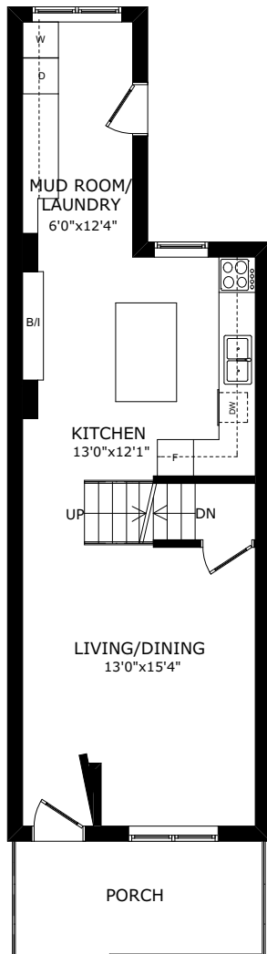
MAIN FLOOR
