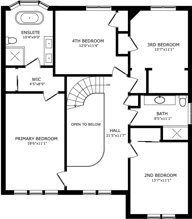
UPPER LEVEL
